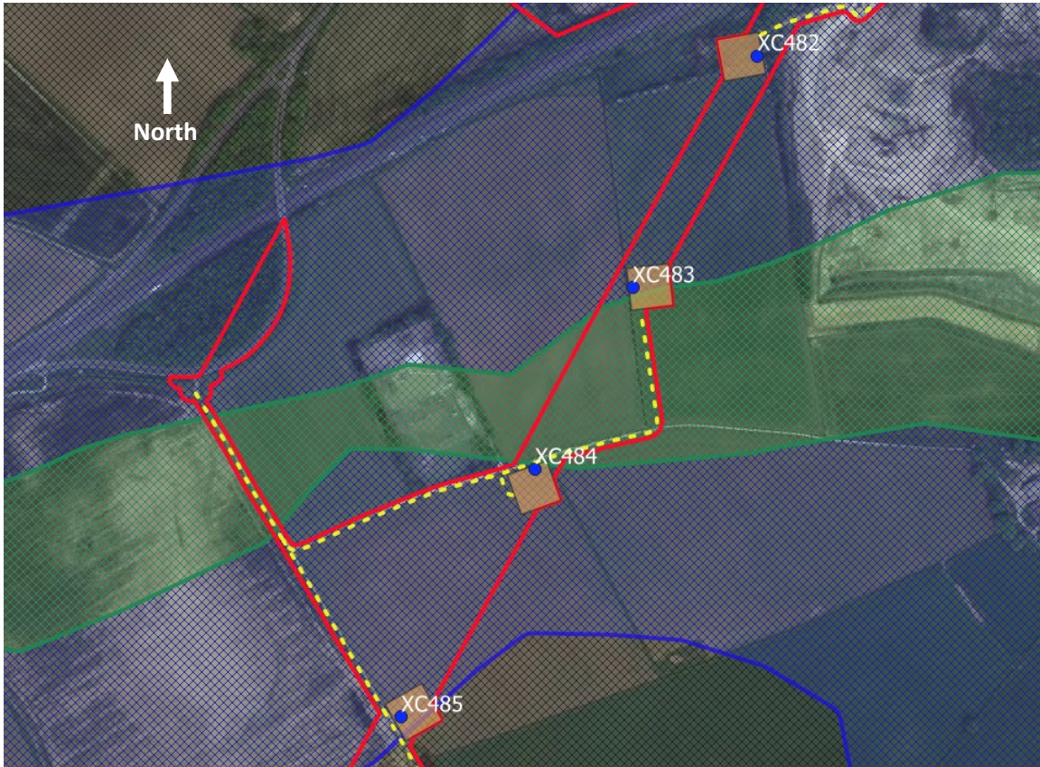
Figure 10.17 - Configuration of works relative to SPZ1
