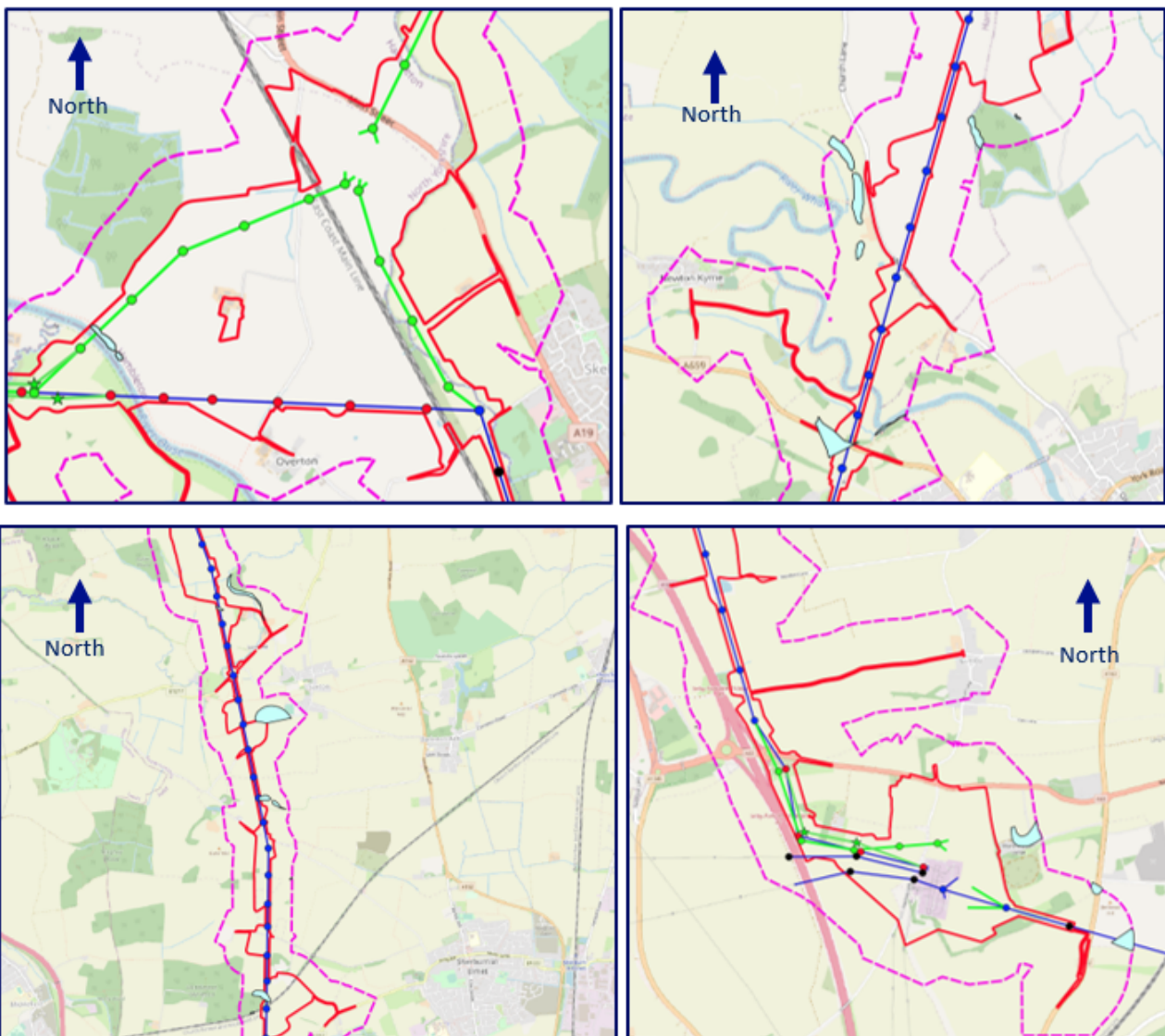
Figure 10.18 – Landslide Hazard Areas
