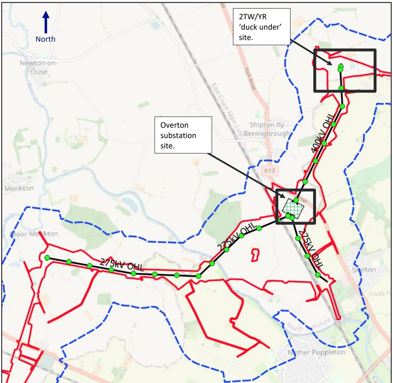
Figure 10.5 - North West of Area
