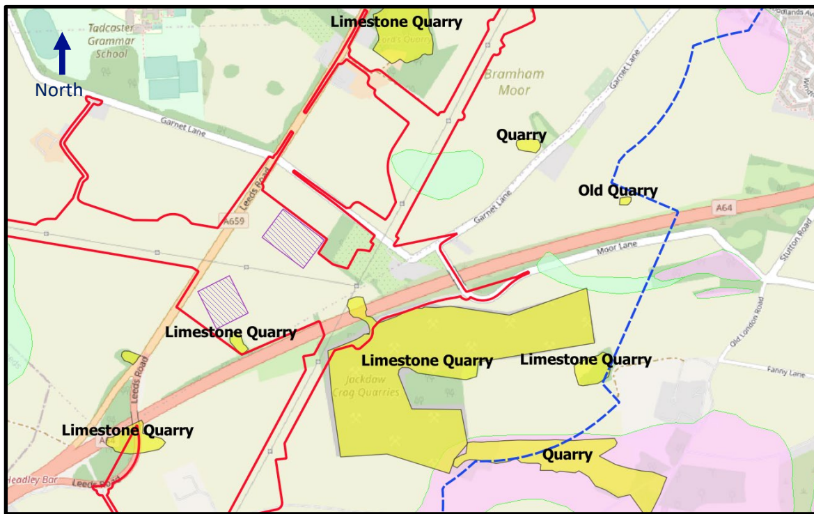
Figure 10.15 - Potential ground gas sources (yellow) near to the proposed Tadcaster Area compounds (purple hatched)
