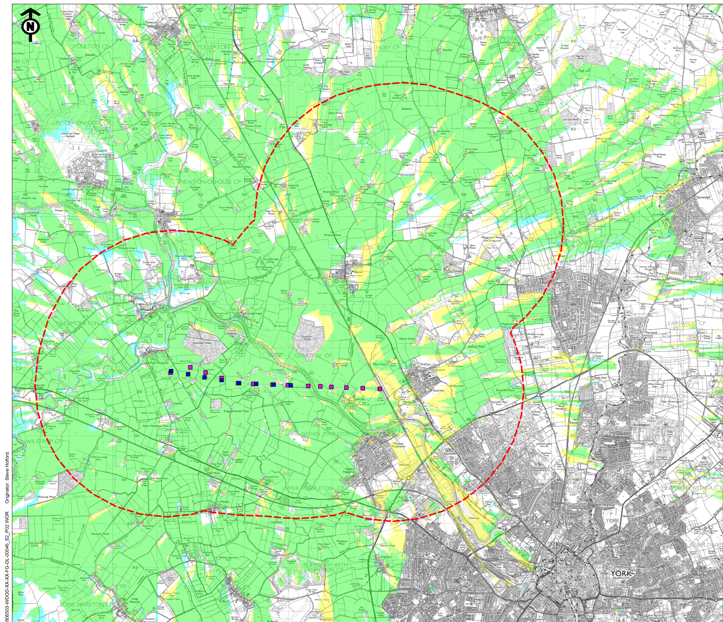
Yorkshire GREEN Project Figure 6.7 Comparative Zone of Theoretical Visibility of North-west of York Area Existing Towers (XCP001-13 & XC429) with Replacement Towers (XC422-429) September 2021
