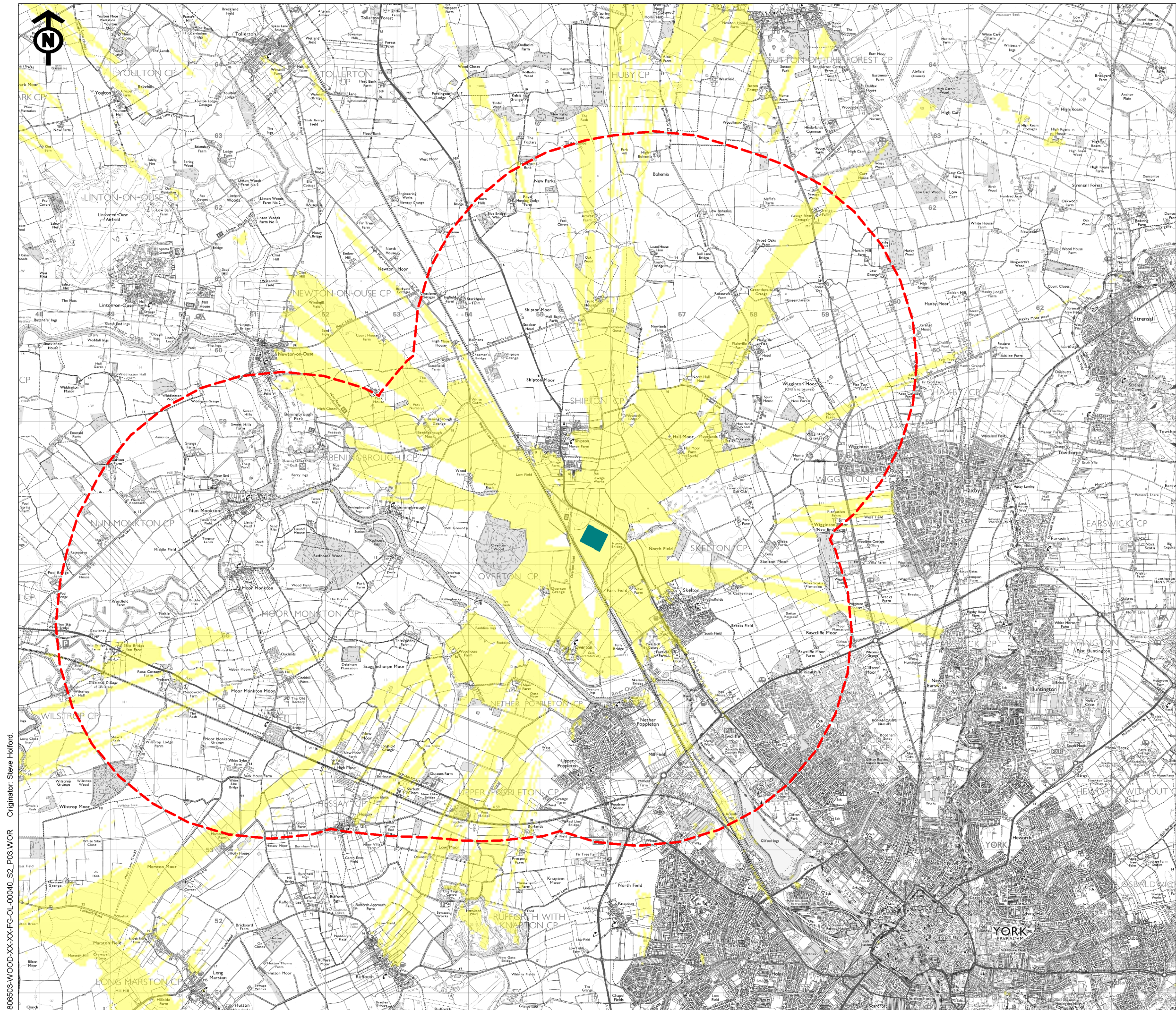
Figure 6.6 Zone of Theoretical Visibility of Overton Substation
