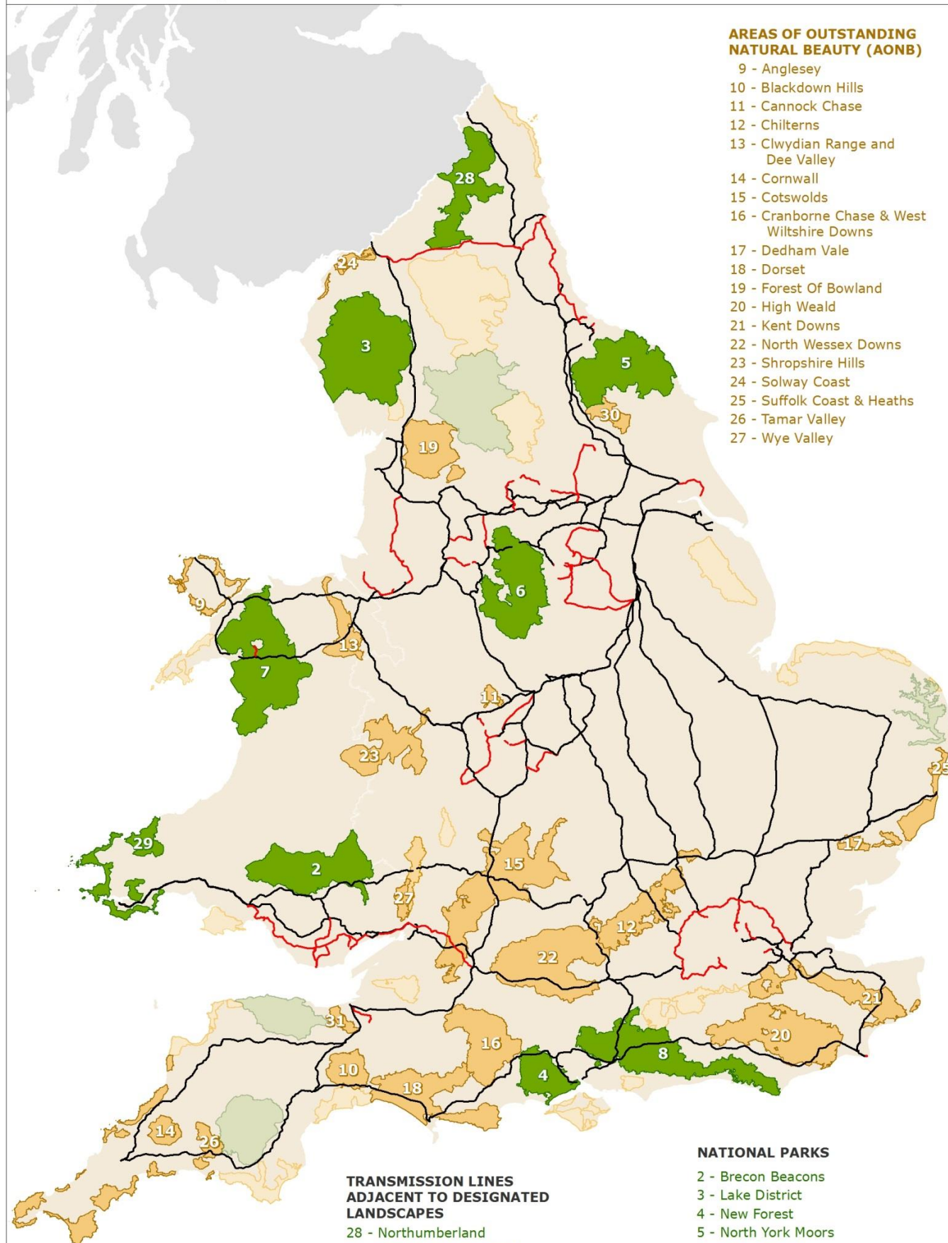
Figure 1: National Grid Transmission Infrastructure and Designated Landscapes
