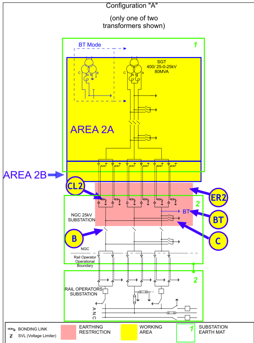
Figure 4.3A – Example of safe working arrangement diagrams
