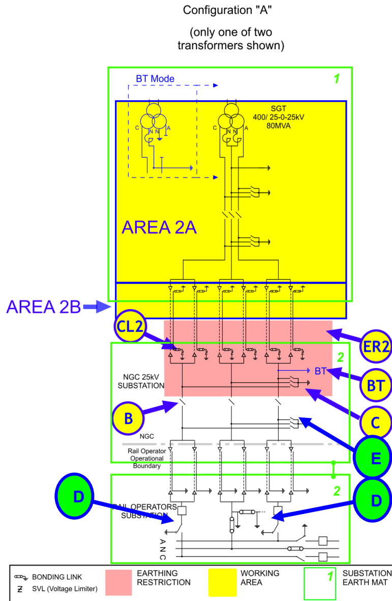
Figure 4.4 An example of Point(s) of Isolation on the neutral conductor only.
