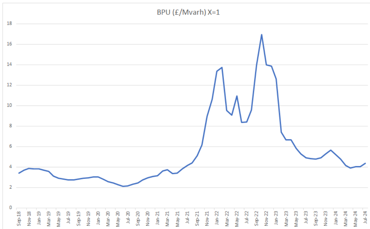
Figure 5.1 – ESO data from the Obligatory Reactive Power Service concerning Cost of Procuring Reactive Compensation
