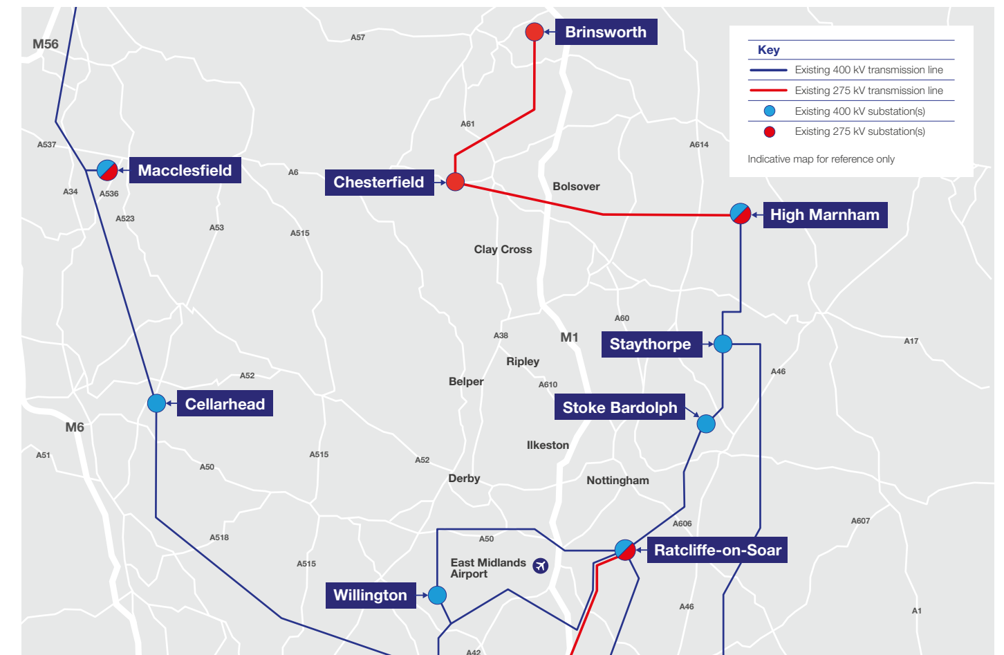
Figure 1: Existing transmission system in the East Midlands region.
