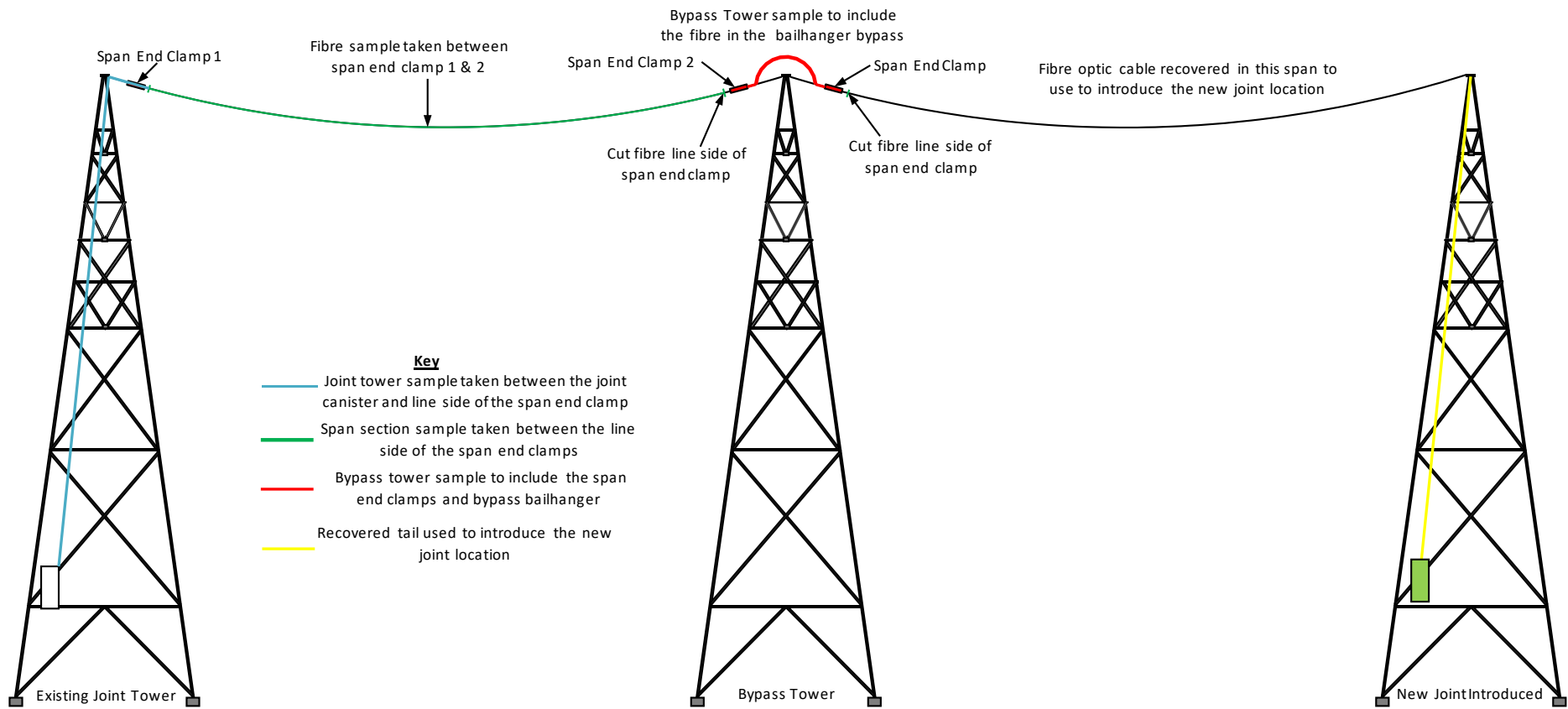
Figure 1 - AFL/Focas Fibre Installation Samples
