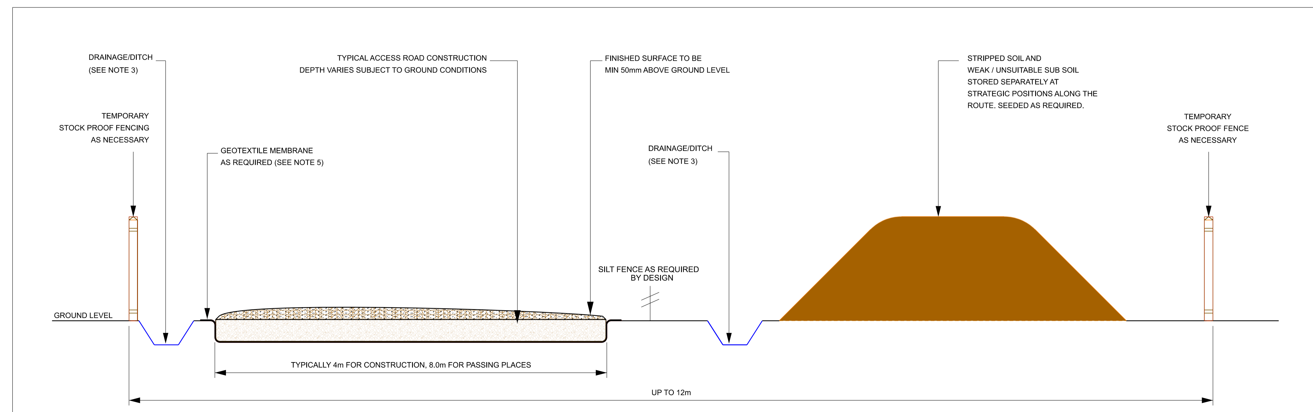
TYPICAL ACCESS ROAD CROSS SECTION
