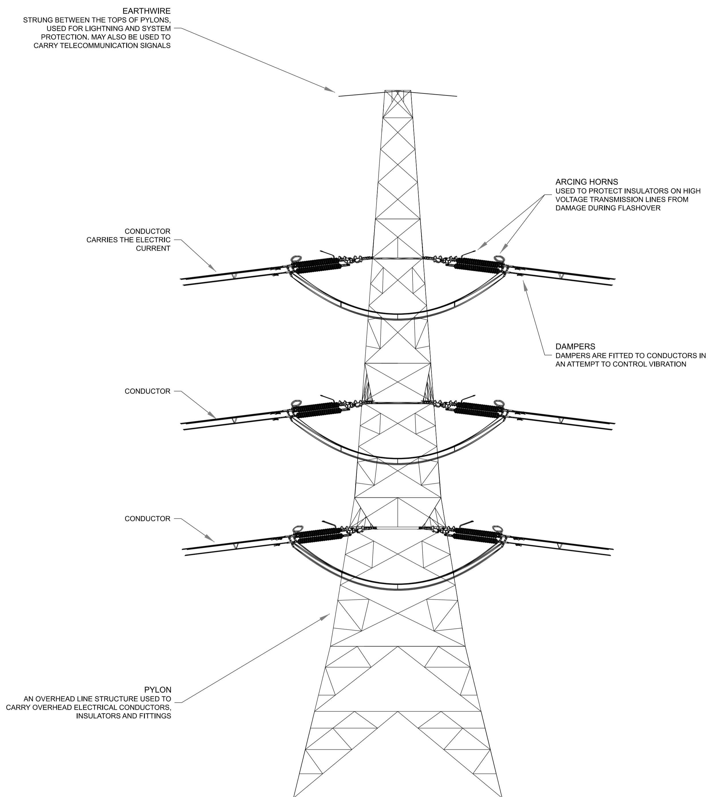
LONGITUDINAL VIEW ON PYLON L12 D90 STD
