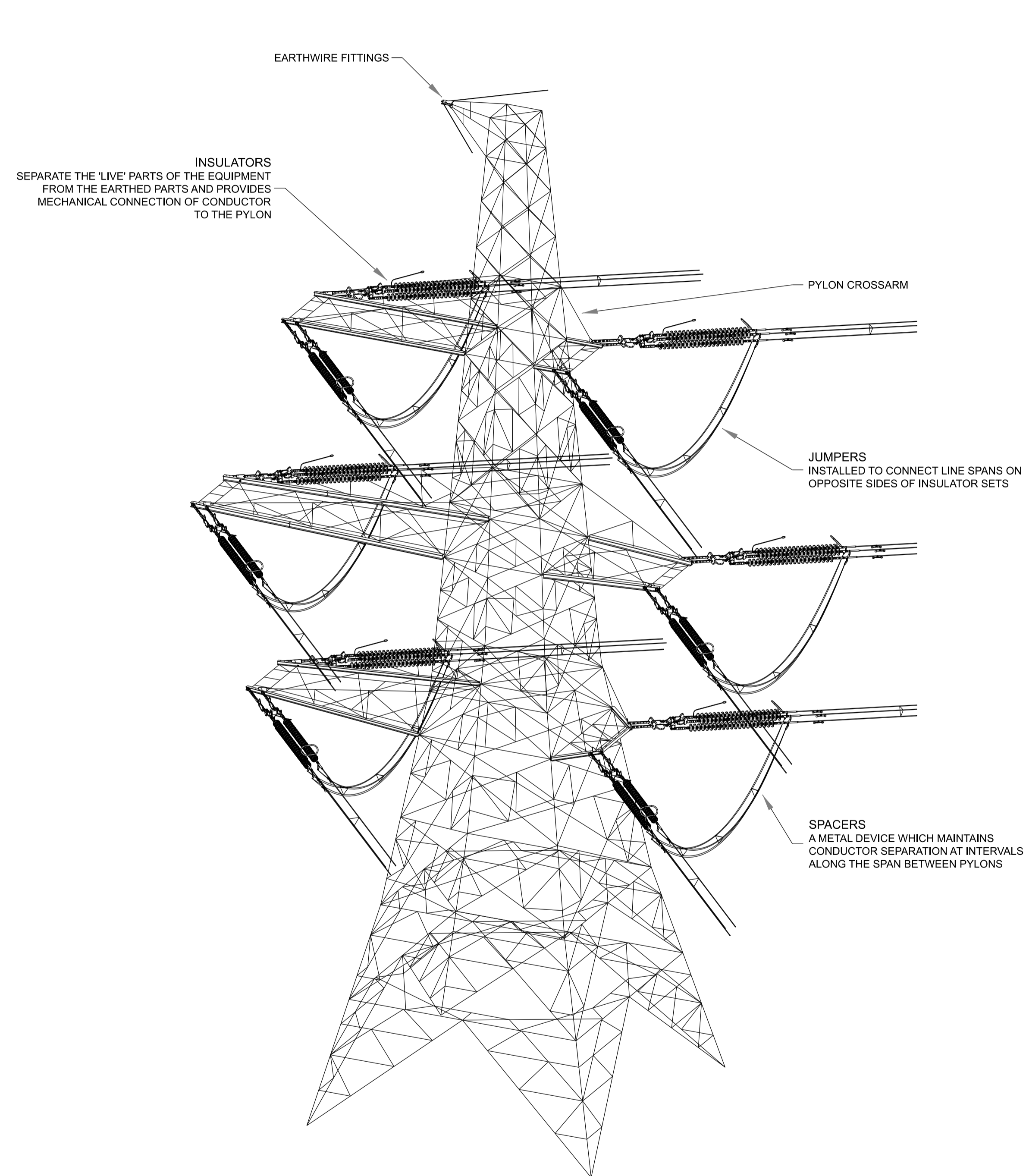
ISOMETRIC VIEW ON PYLON L12 D90 STD
