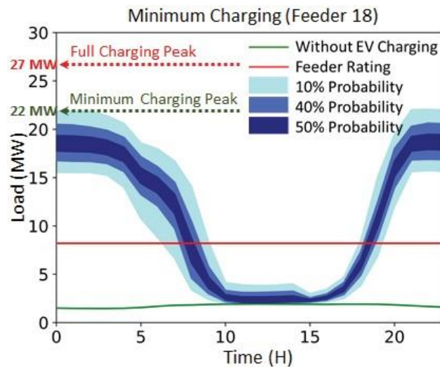
Figure 15: Reduction in the peak load duration through minimum charging strategy
