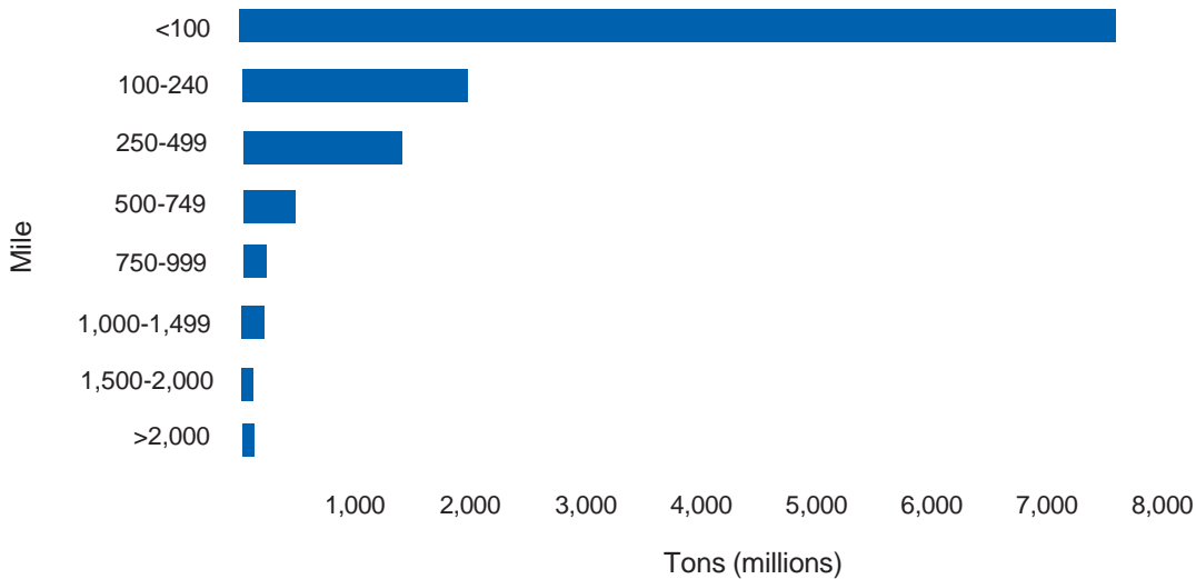
Figure 2: Truck Freight (by Weight) by Distance Traveled
