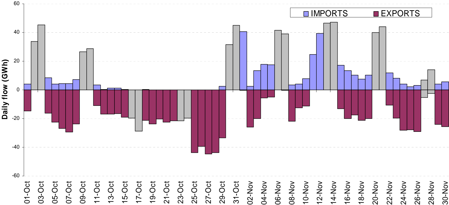
Flows over the French English Interconnector October - November 2010
