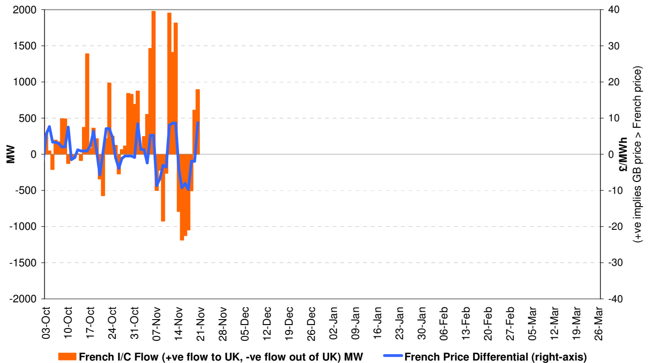
French Interconnector Flow and French Price Differential (3 - 7 pm)
