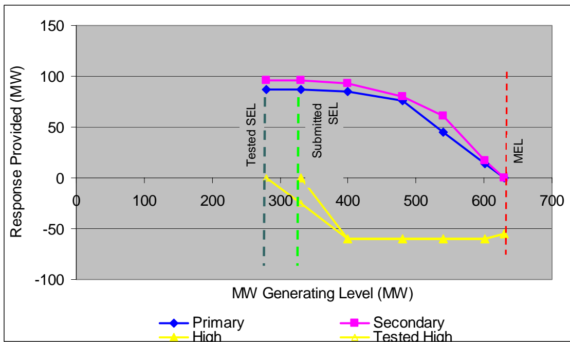
Figure 6 Option 4 anchor capability to fixed SEL with option to change to submitted SEL
