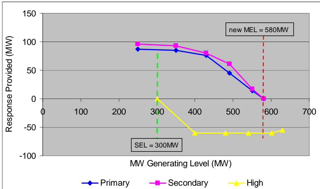
Figure 3 Option 1 Anchor HF capability at SEL: no change to LF capability
