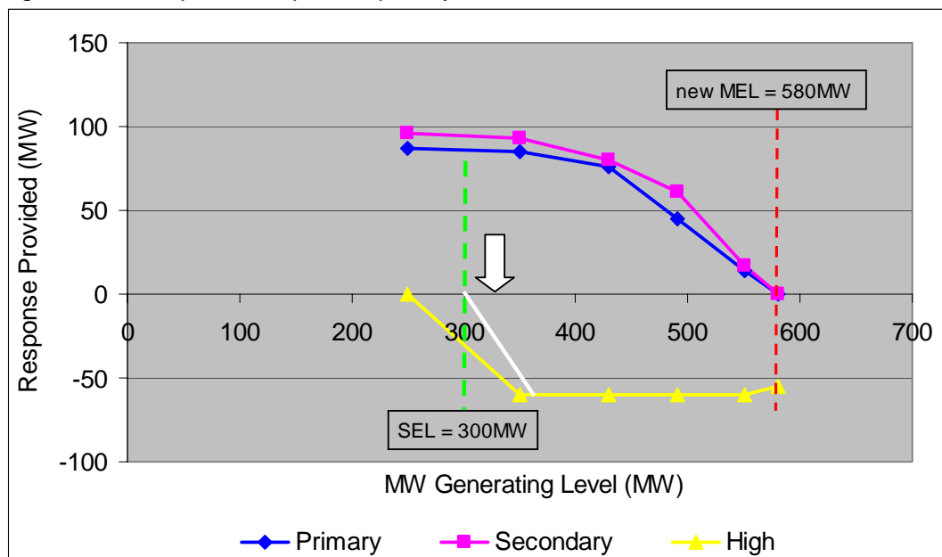
Figure 4 Option 2 Cap HF capability at x-SEL
