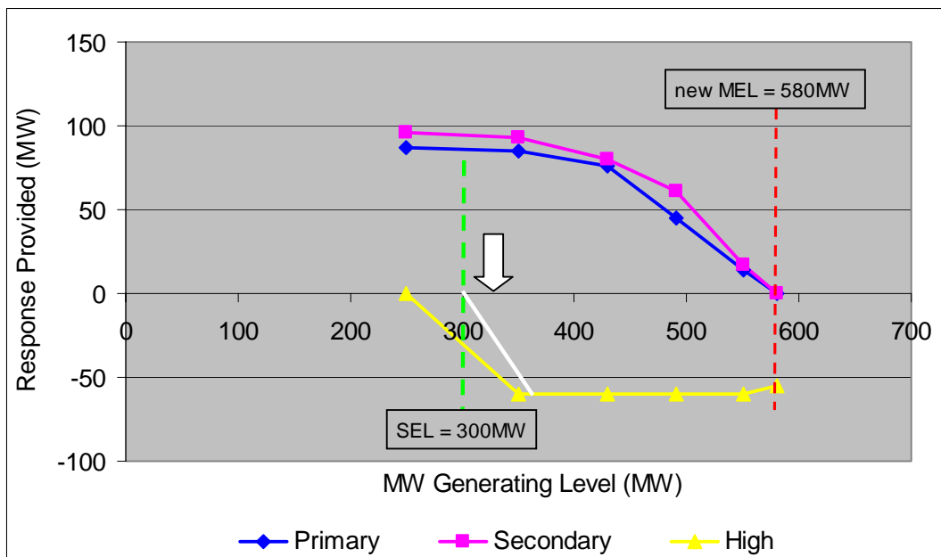
Figure 2 MEL redeclared to 580MW from 630MW
