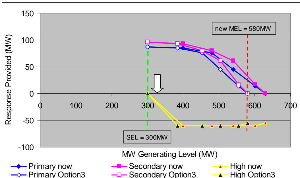
Figure 5 Option 3 compress the response curves between declared MEL and SEL
